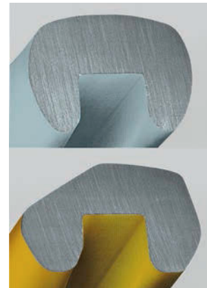
Comparison of the scarf cross-section in a standard needle (above) and a SAN@ 6 GEBEDUR@ needle (below)
